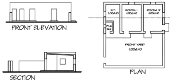
DWELLING UNIT 4
