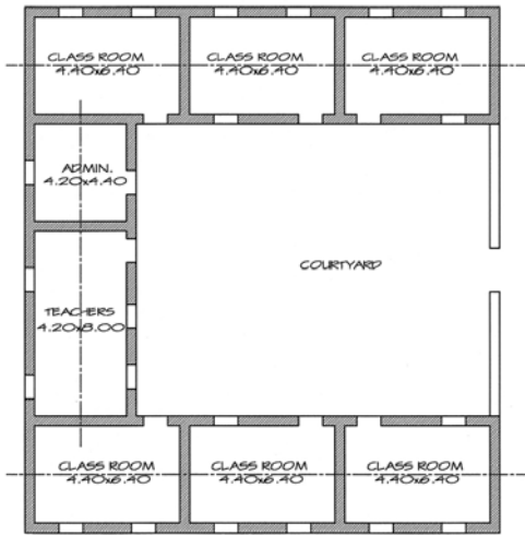
PLAN SCHOOL
